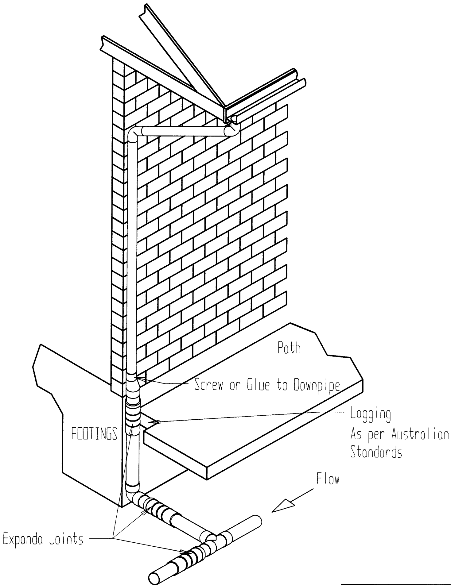
GUIDELINES FOR PVC-U DRAINAGE SYSTEM WITH EXPANSION JOINT LOCATIONS FOR REACTIVE SOILS
